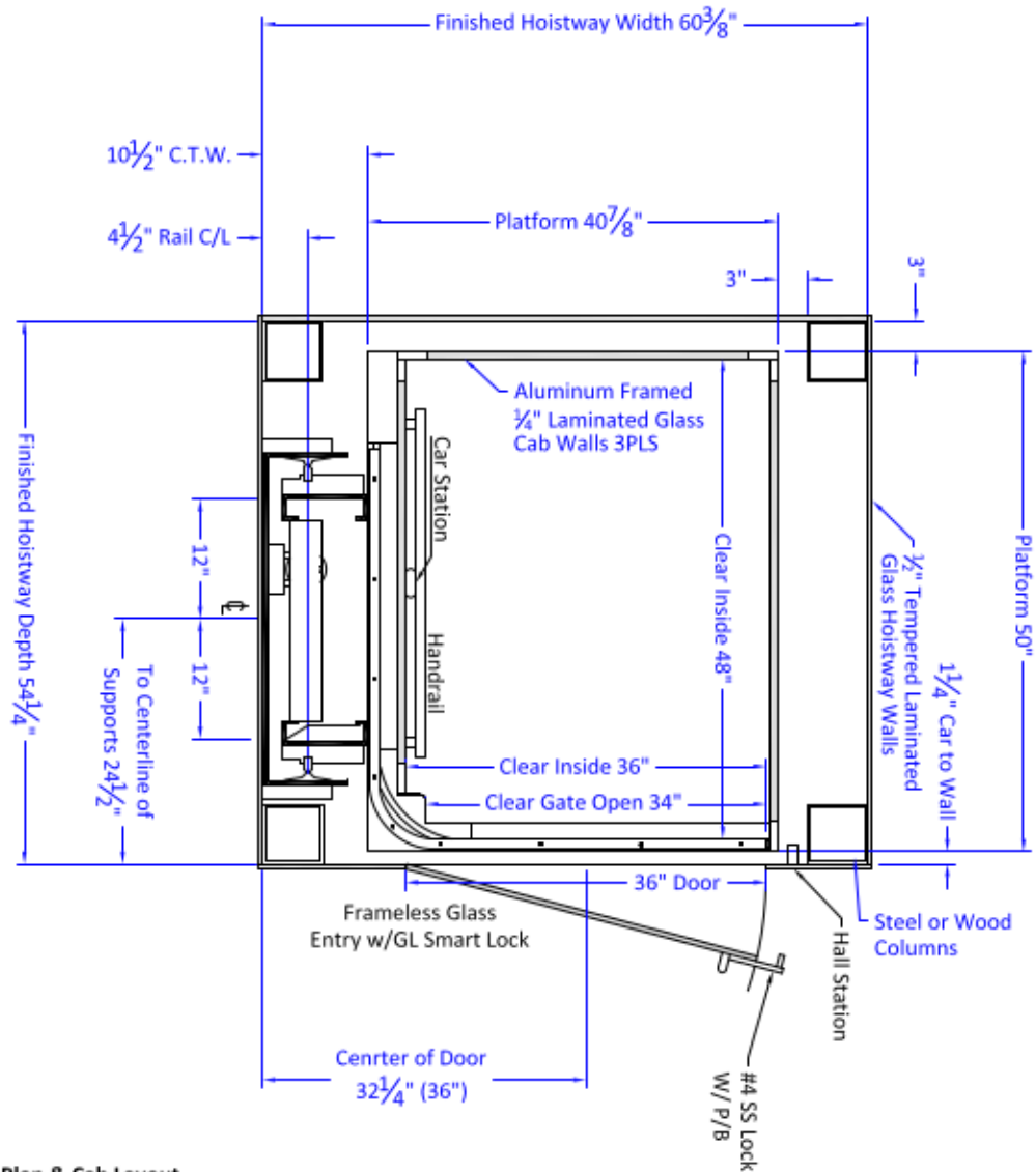
Floor Plan & Cab Layout 950# CAPACITY WRAP-AROUND GATE & SWING LANDING DOORS
