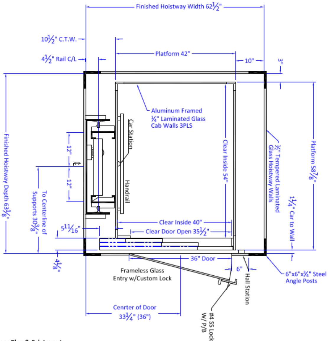
Floor Plan & Cab Layout 950# CAPACITY VICTORY 3-SPEED CAR DOORS w/POCKET & SWING LANDING DOOR
