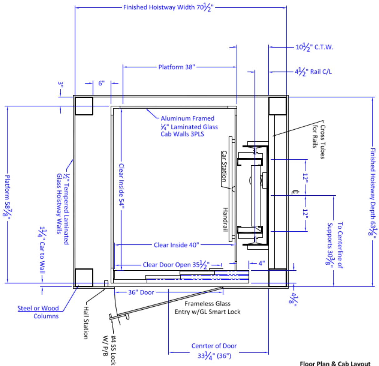
Floor Plan & Cab Layout 950# CAPACITY VICTORY 3-SPEED CAR DOORS w/POCKET & SWING LANDING DOOR
