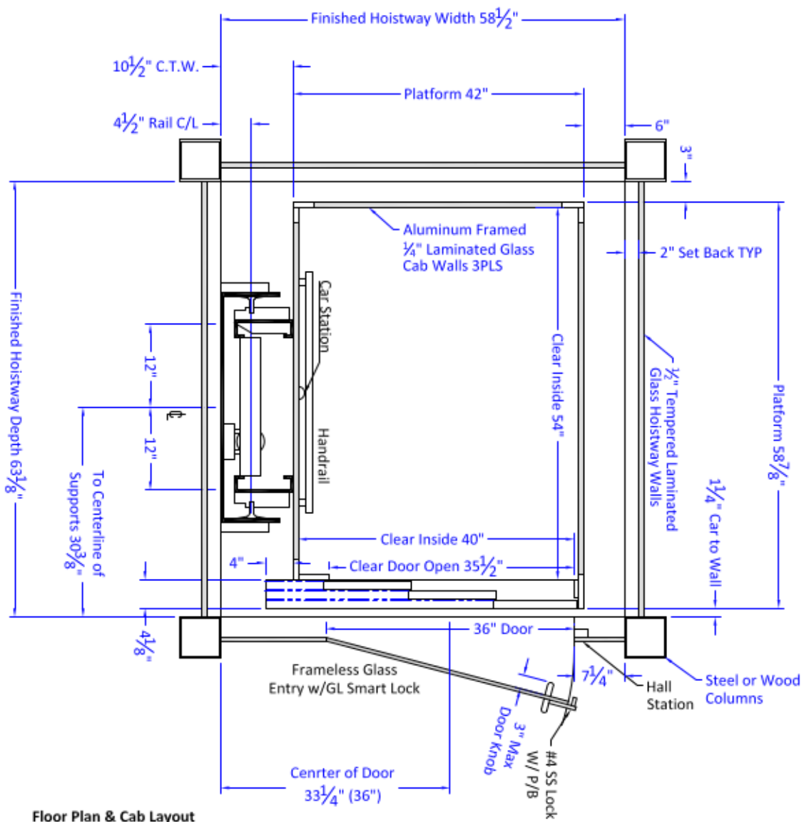
Floor Plan & Cab Layout 950# CAPACITY VICTORY 3-SPEED CAR DOORS w/POCKET & SWING LANDING DOOR
