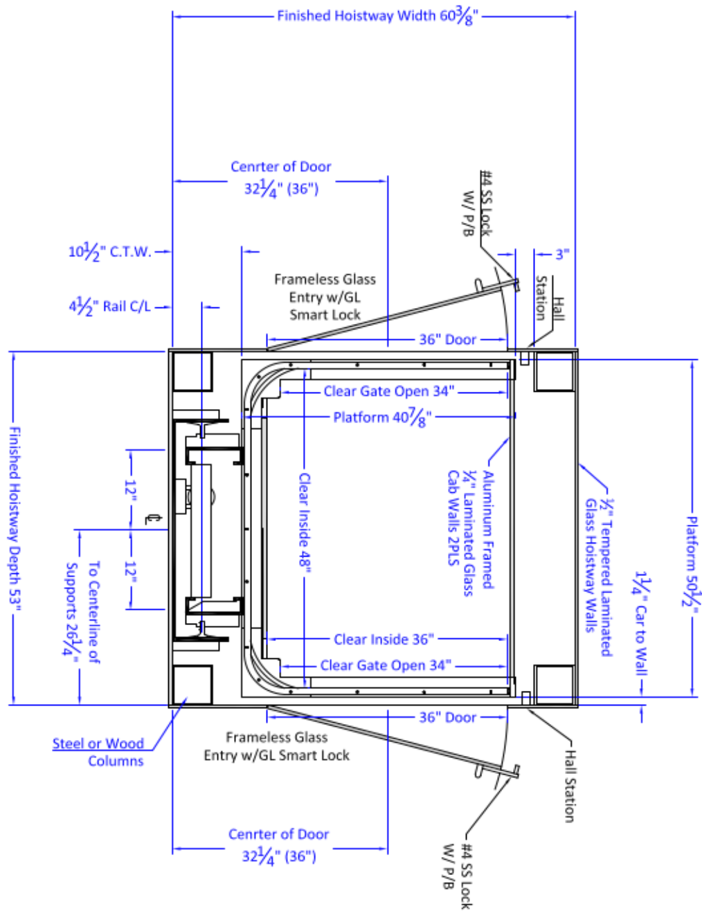
Floor Plan & Cab Layout 950# CAPACITY WRAP-AROUND GATES & SWING LANDING DOORS
