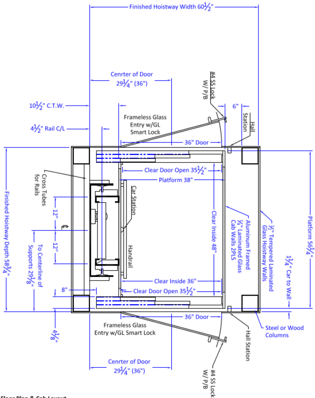
Floor Plan & Cab Layout 950# CAPACITY VICTORY 3-SPEED CAR DOORS w/POCKET & SWING LANDING DOOR
