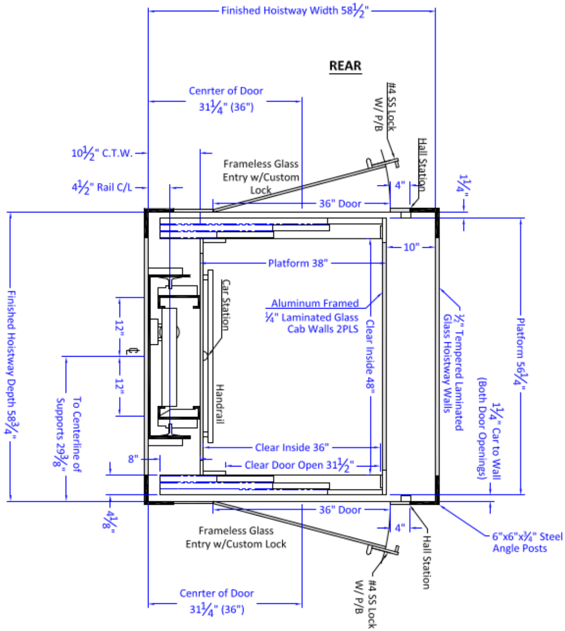
Floor Plan & Cab Layout 950# CAPACITY VICTORY 3-SPEED CAR DOORS w/POCKET & SWING LANDING DOOR
