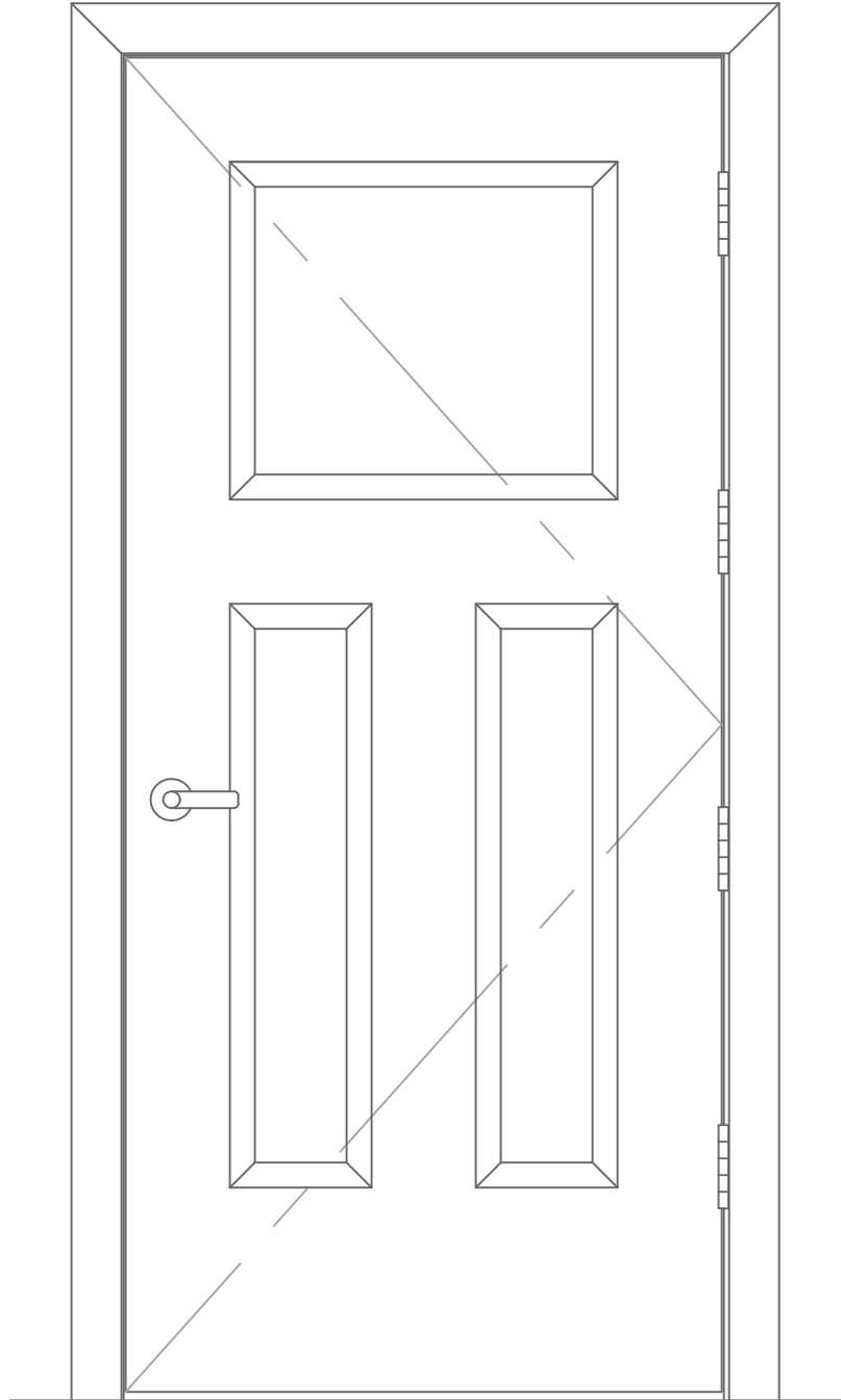
1 - 3 RAISED PANEL MISSION DOOR SCALE: 1" = 1'-0"
