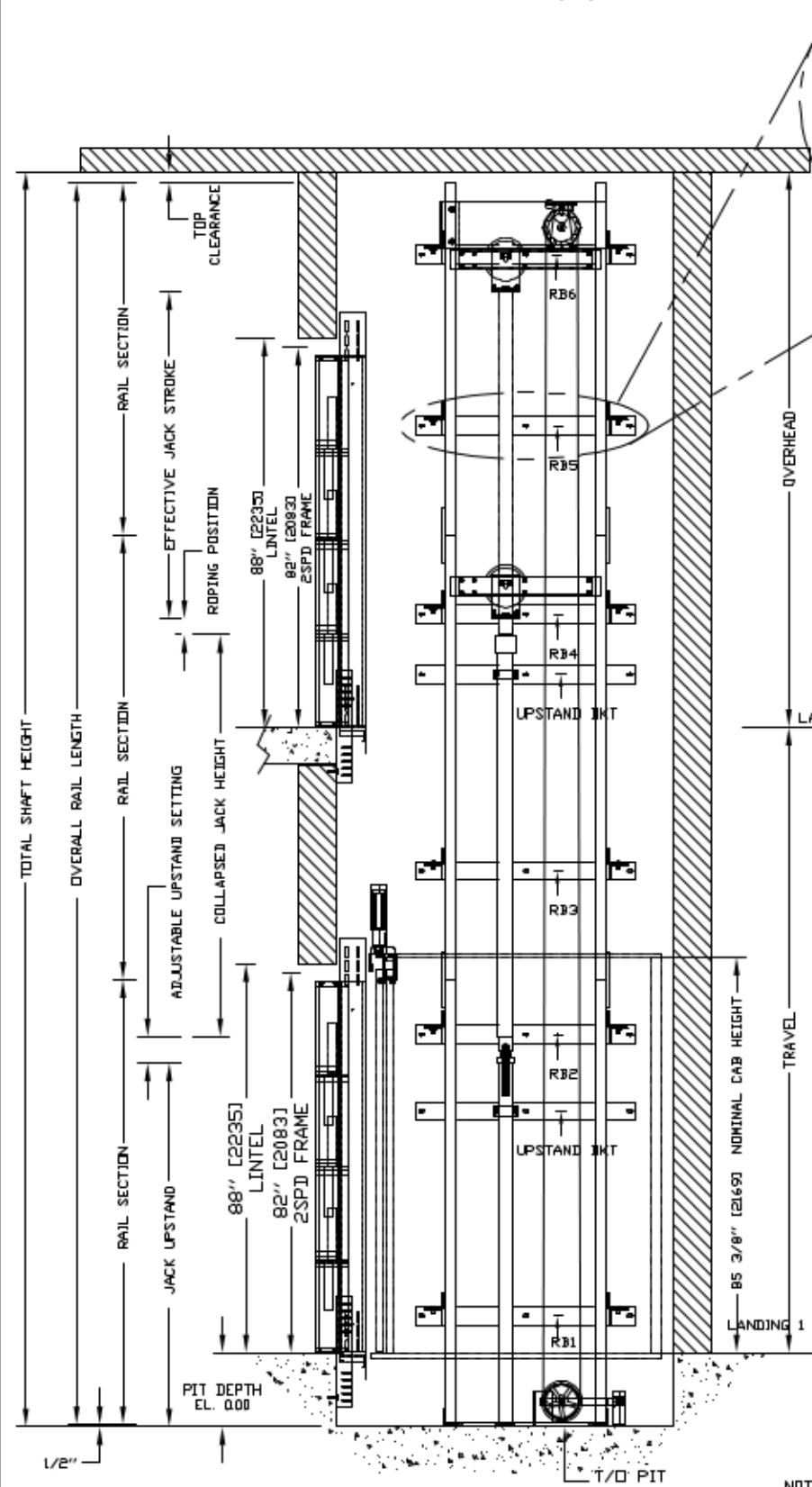
SECTIONAL VIEW - ORION-4854 (1L)
