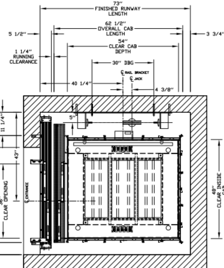
PLAN VIEW - ORION17-4854 (1L) 2 SPEED WITTUR DOORS
