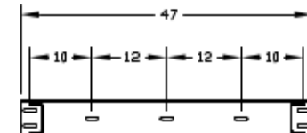
RAIL BRACKETS
