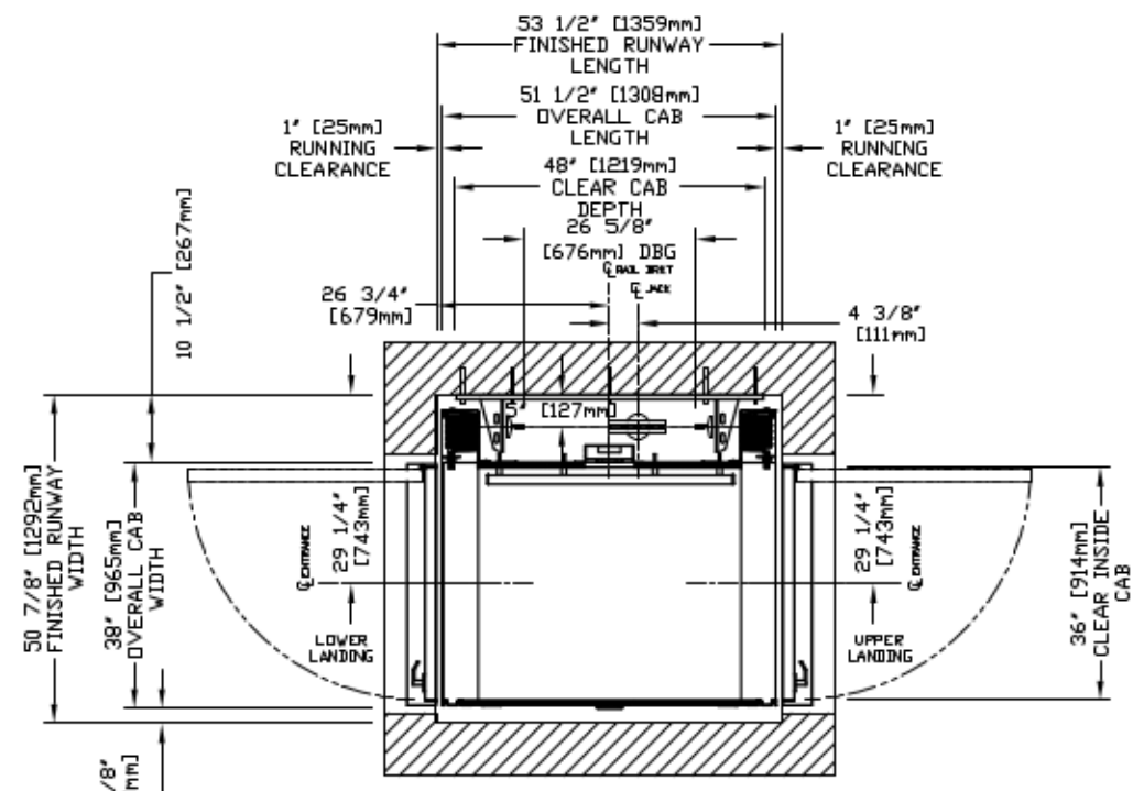
RAIL BRACKET
