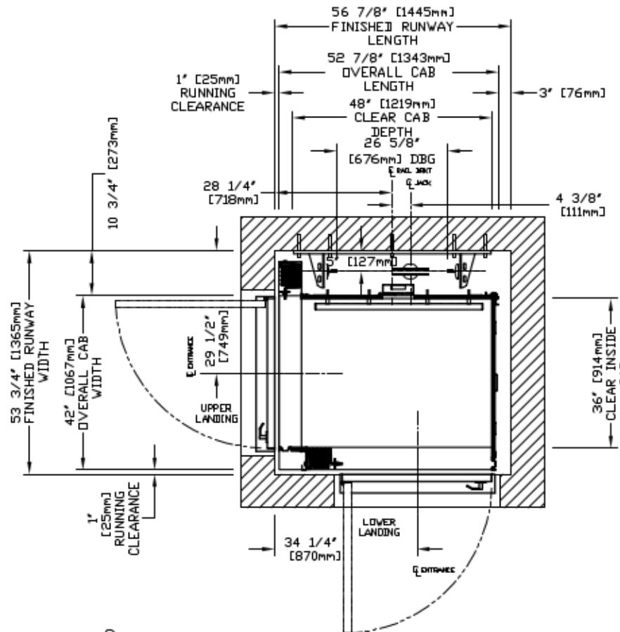
RAIL BRACKET PLAN VIEW - INFINITY Model 3648 TYPE 4
