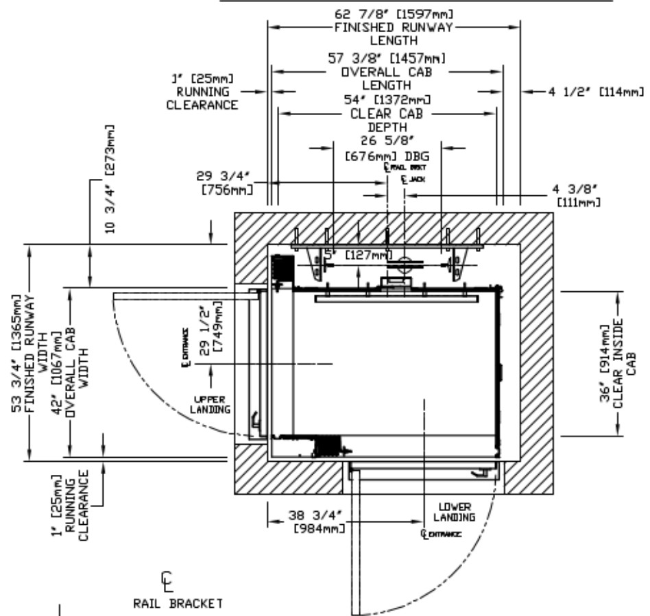
RAIL BRACKET PLAN VIEW - INFINITY Model 3654 TYPE 4
