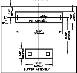
RAIL BRACKET
