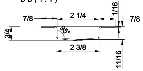
B-B (1:1)
