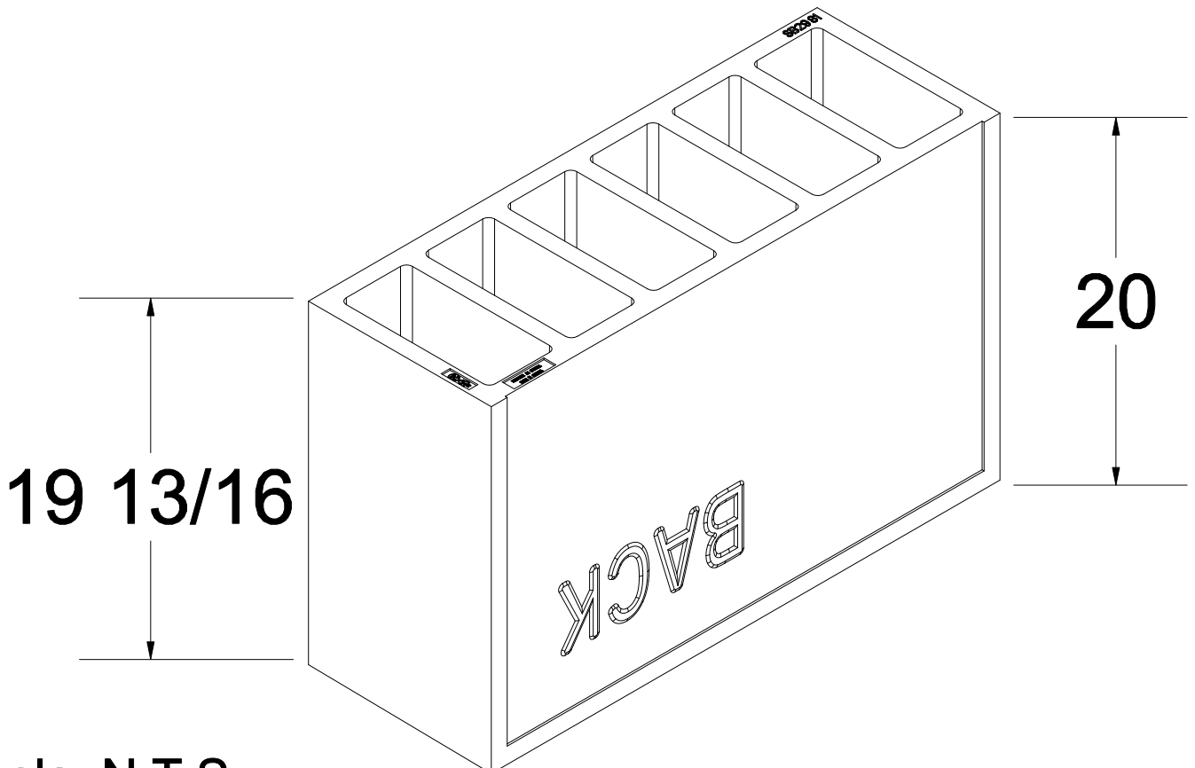
Underside view
