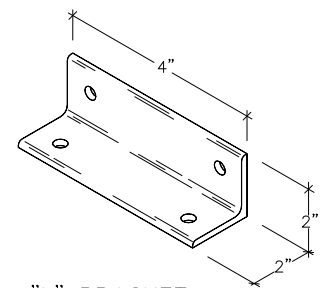
"L" BRACKET N T S
