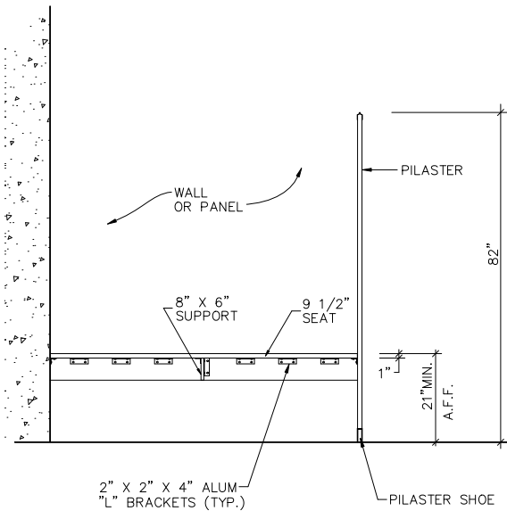
STD. SHOWER SEAT ELEVATION N T S
