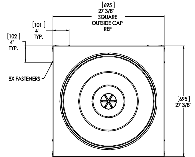
TOP VIEW SCALE 1:1
