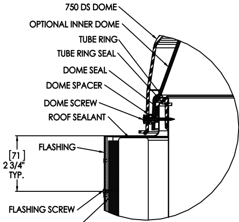
DETAIL B SCALE 3 : 1
