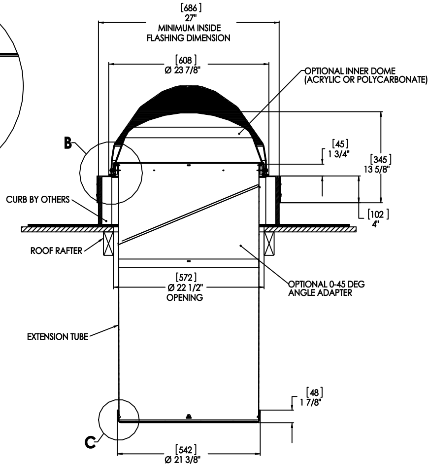
FULL SECTION SCALE 1:1
