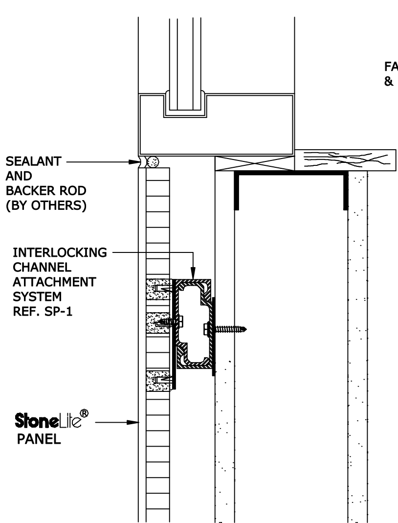
FLUSH WINDOW SILL
