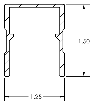
DETAIL C SCALE 1 : 1
