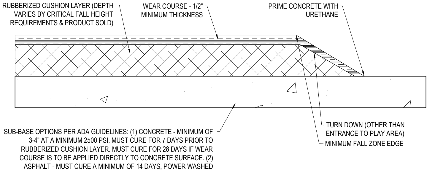
SECTION VIEW
