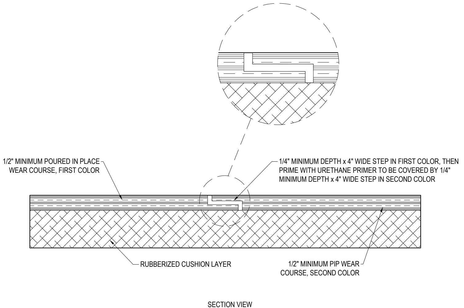
SECTION VIEW
