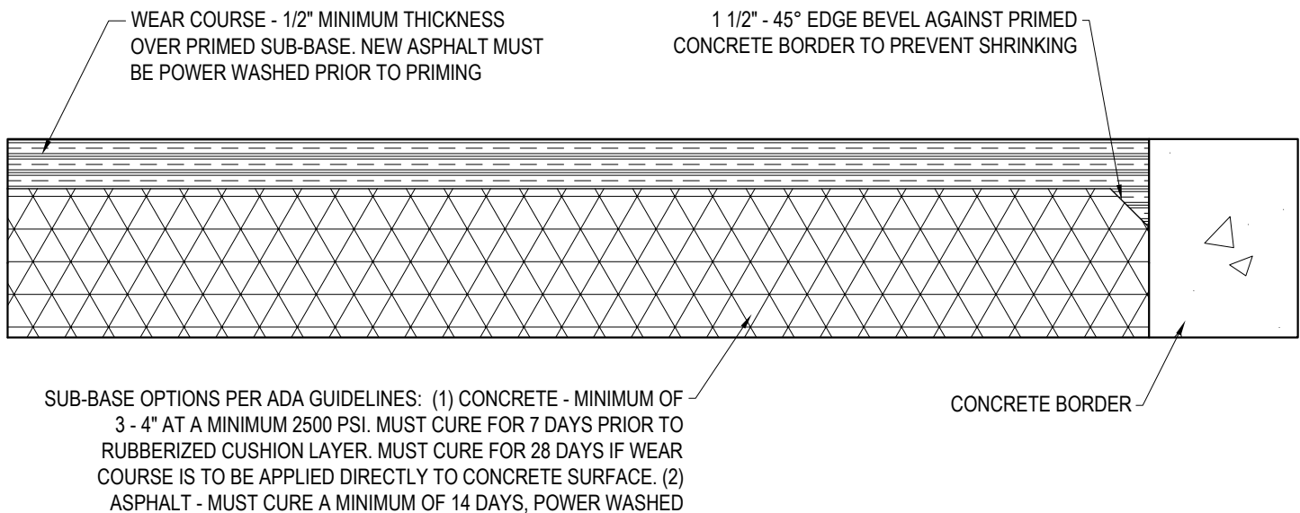
SECTION VIEW
