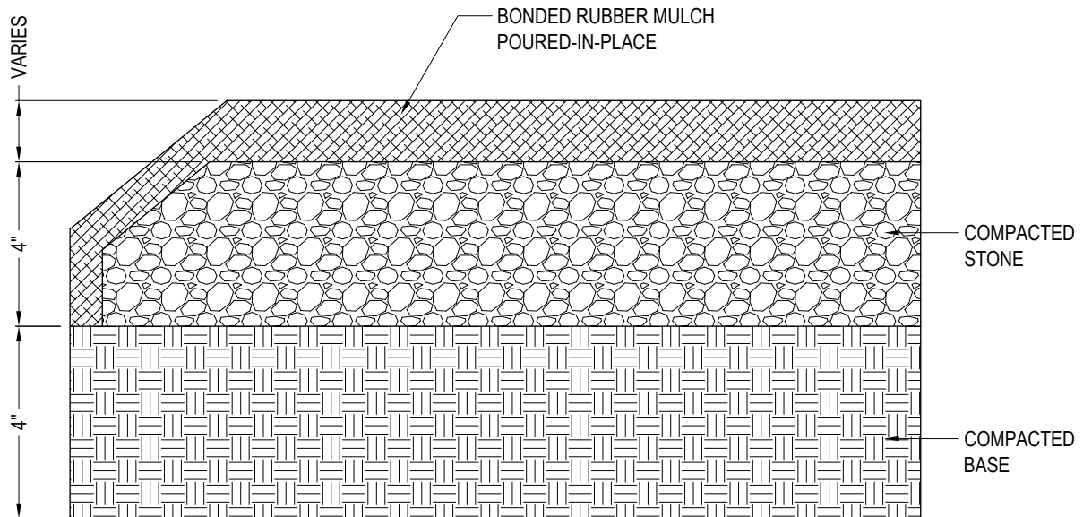
SECTION POUR-IN-PLACE ON COMPACTED CRUSHED STONE BASE
