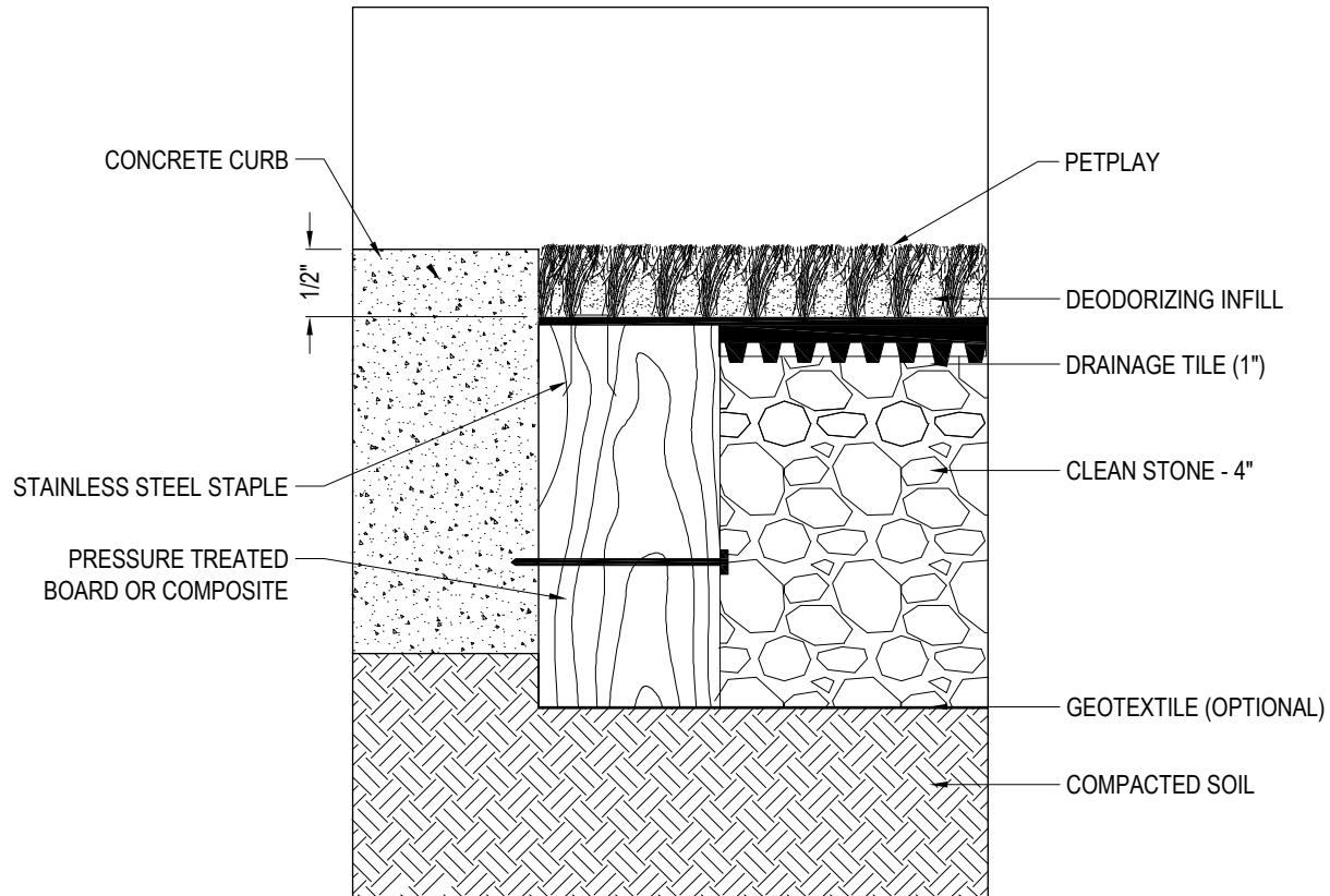
SECTION VIEW INSTALLATION WITH CURB
