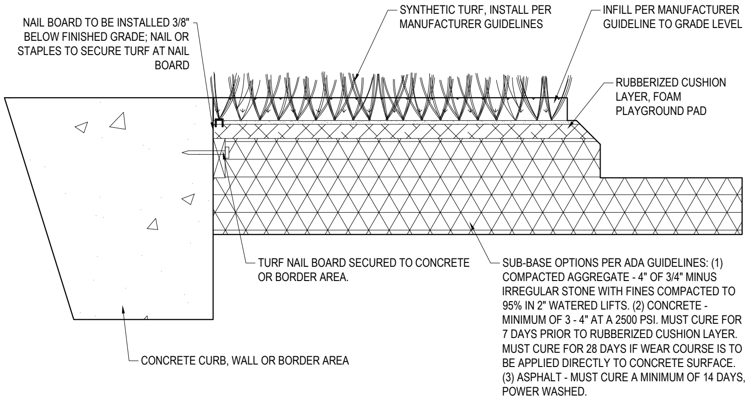
SECTION VIEW
