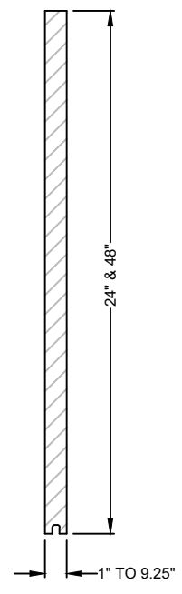
SECTION
