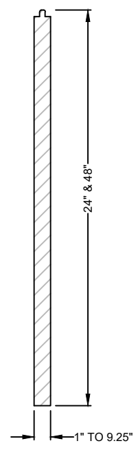
SECTION
