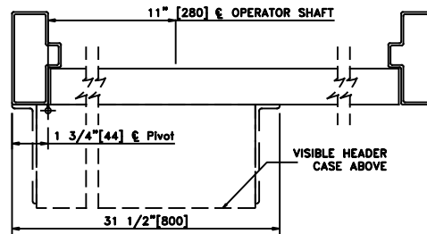
① HORIZONTAL SECTION
