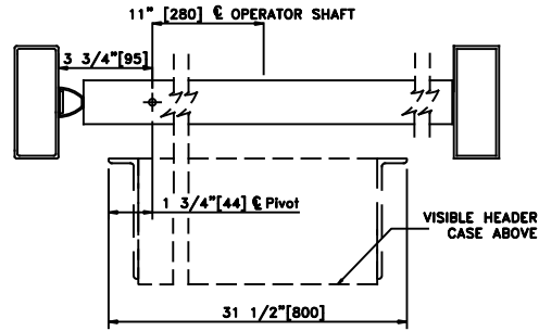
① HORIZONTAL SECTION
