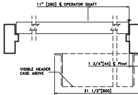
① HORIZONTAL SECTION
