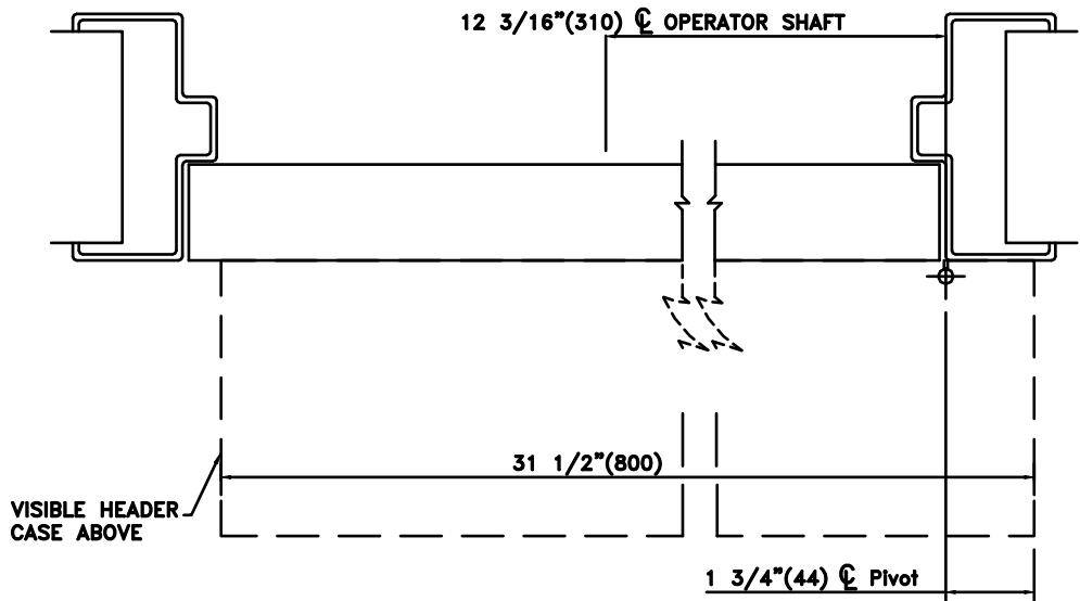
2 HORIZONTAL SECTION
