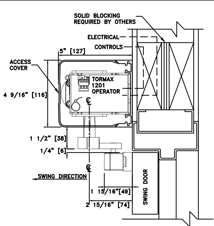
1 VERTICAL SECTION
