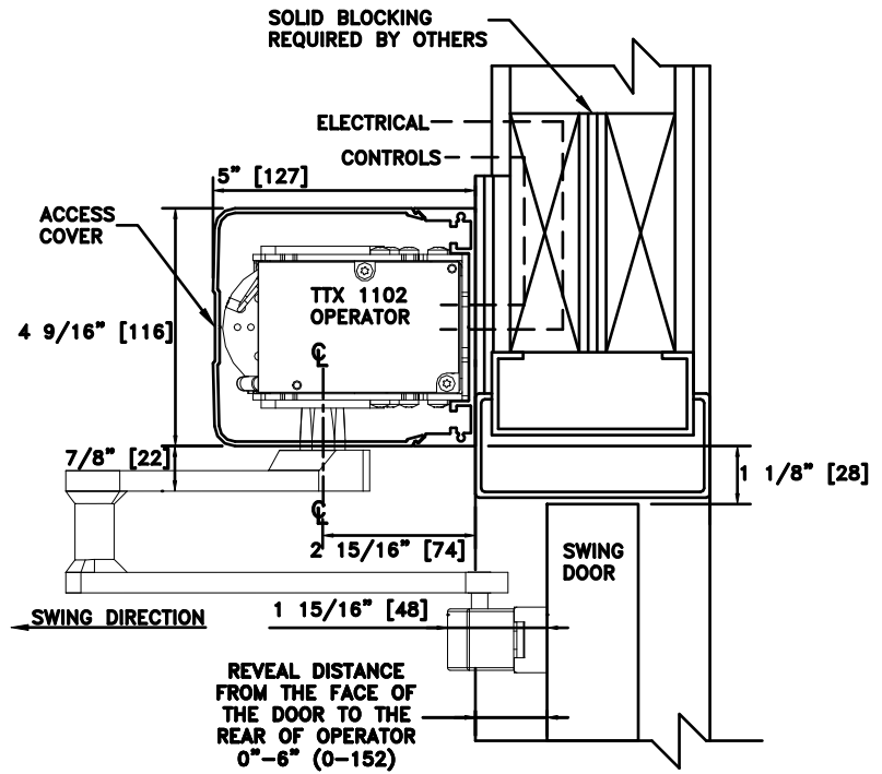
1 VERTICAL SECTION
