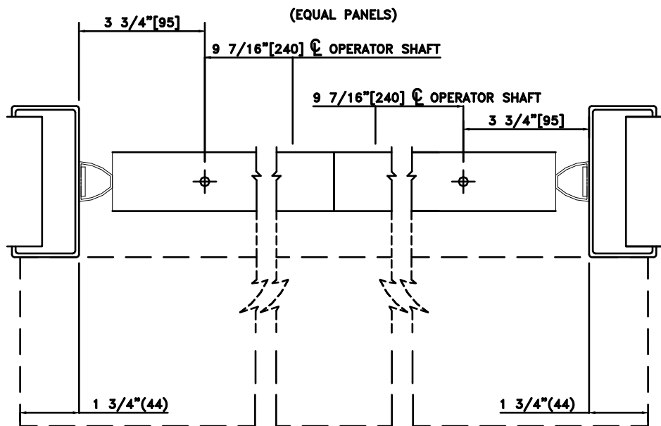
2 HORIZONTAL SECTION
