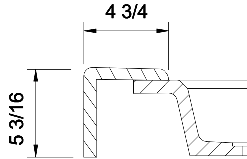
THRESHOLD DETAIL
