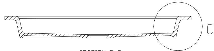
SECTION B-B
