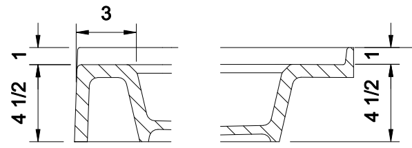
DETAIL C
