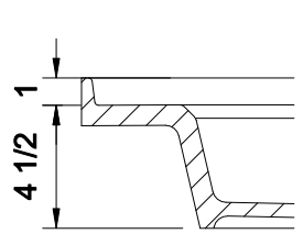
DETAIL C
