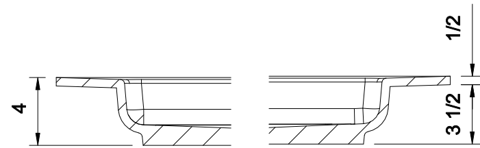
DETAIL D DETAIL C
