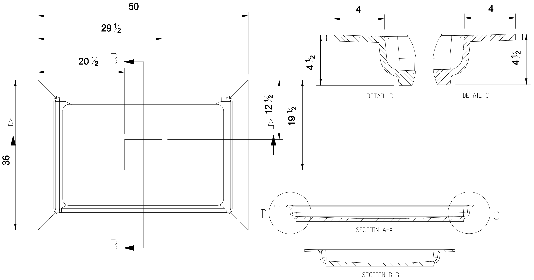
Tower Industries Meridian Solid Surface Shower Base Model #: MSB5036SUV
