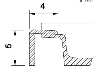
THRESHOLD DETAIL
