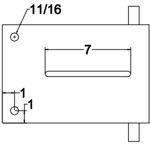
Mounting Plate 8" x 12" x 3/8"
