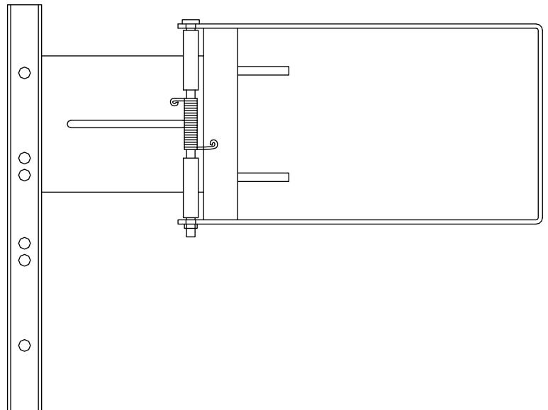
Mounting Channels (2) 24" x 2" x 1"
