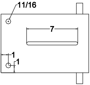
Mounting Plate 8" x 12" x 3/8"
