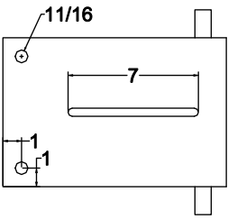
Mounting Plate 8" x 12" x 3/8"
