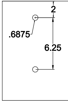
Receiving Plate 12" x 8" x \frac{3}{8} " (By request only - Pipe mount)
