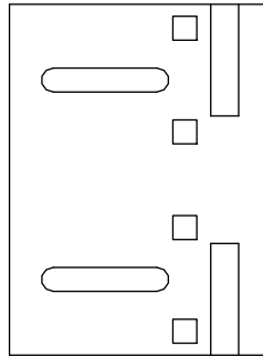
Mounting Plate 11" x 8" x \frac{3}{8} " (2) 4" x \frac{3}{4} " Slots (4) \frac{3}{4} " Square Bolt Holes
