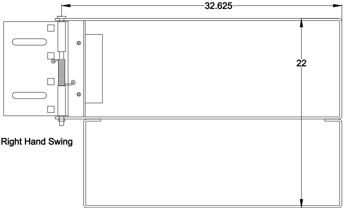
Mounting Plate 11" x 8" x \frac{3}{8} " (2) 4" x \frac{3}{4} " Slots (4) \frac{3}{4} " Square Bolt Holes
