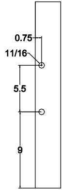
Pipe Post Adapter 22" x 3" x 1/4"
