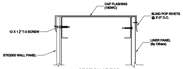
SECTION AT TOP
