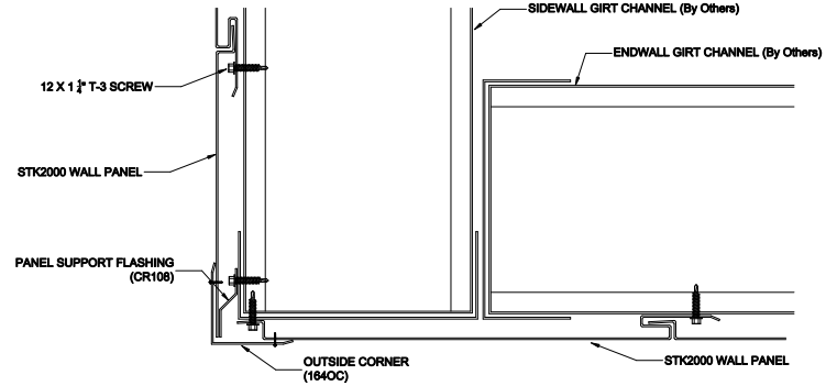
SECTION AT CORNER
