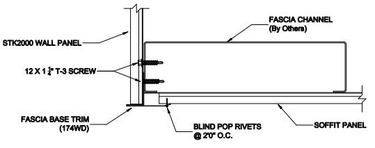
SECTION AT BOTTOM
