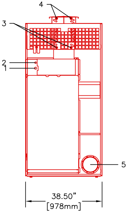
REAR VIEW
