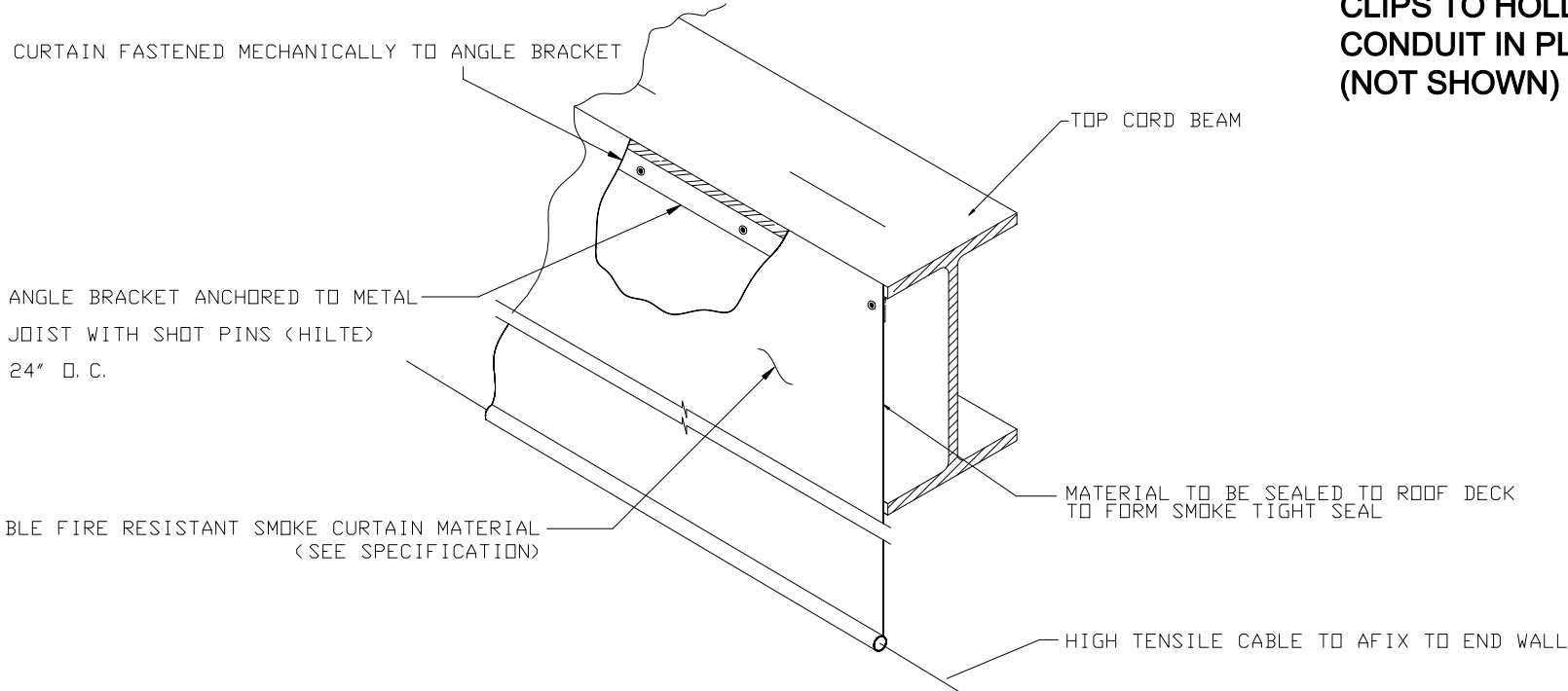
USSF FIXED IN PLACE DRAFT CURTAIN CONNECTION TO BEAM
