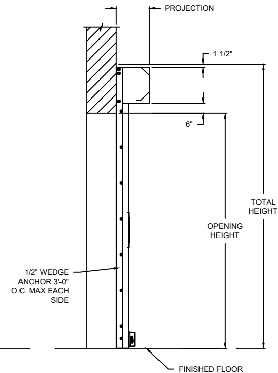
SECTION B-B
