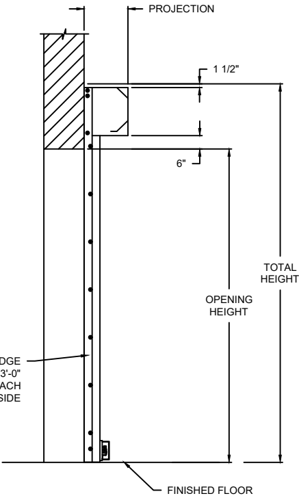
SECTION B-B
