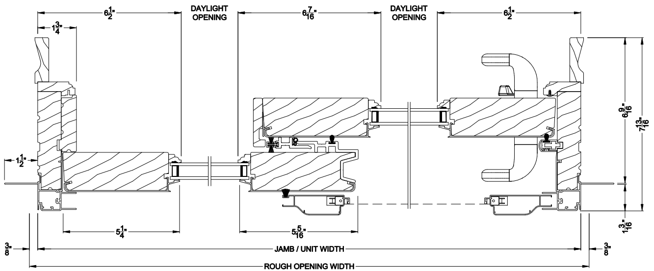
PREMIUM FRENCH SLIDING PATIO DOOR (8715) Horizontal Section - 6-9/16" Jamb
